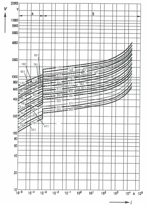
MYE30-201□ ~ MYE30-122□
