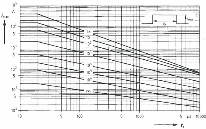
MYE40-201□ ~ MYL40-122□
